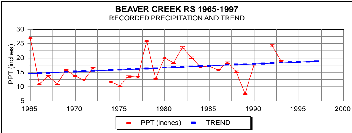
Figure 4.34 Precipitation Trend Analysis
