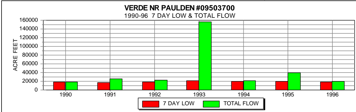
Figure 4.28 Average 7-Day Low Flows & Average Total Flows for 1990-1996
