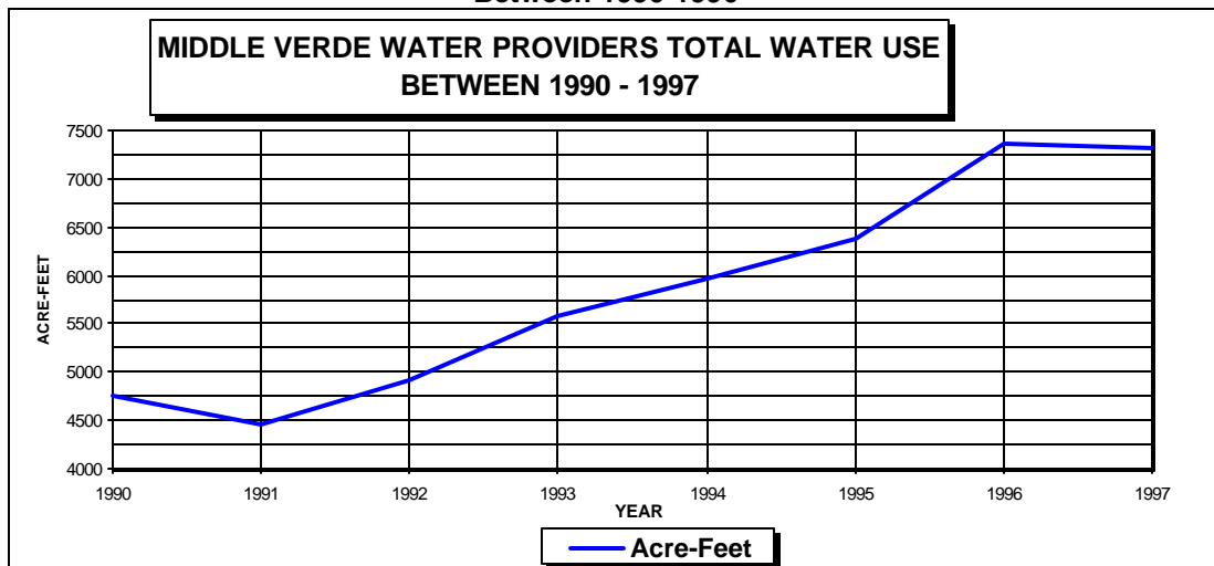
Middle Verde Total Water Use From Water Providers Between 1990-1996
