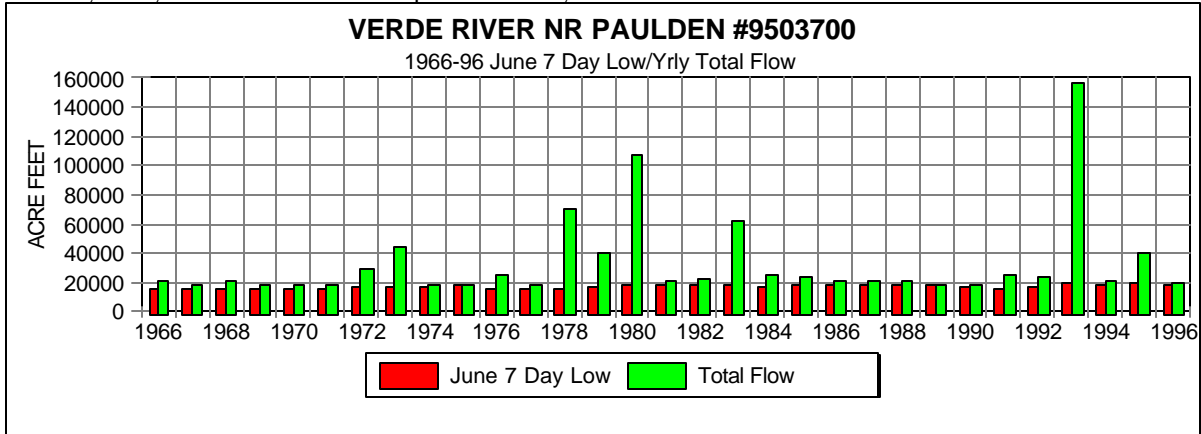
Figure 4.29 Historical June 7-Day Low Flows & Total Flows
