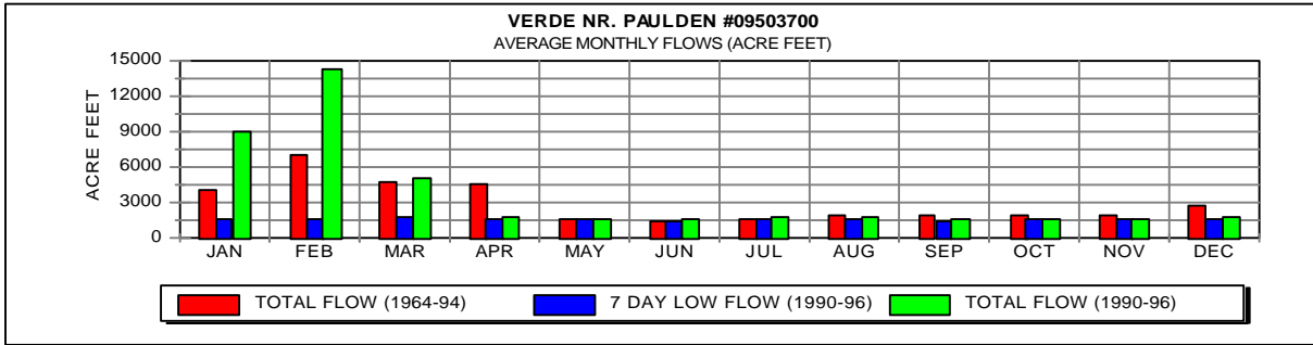
Figure 4.32 Mean 7-day Low Flows and Average Total Flows; Historical and 1990-96
