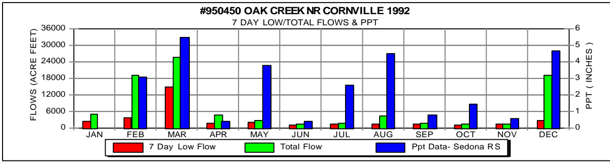
Figure 4.31 Gaged Stream Flow and Precipitation Station Comparisons- 1992 & 1996
