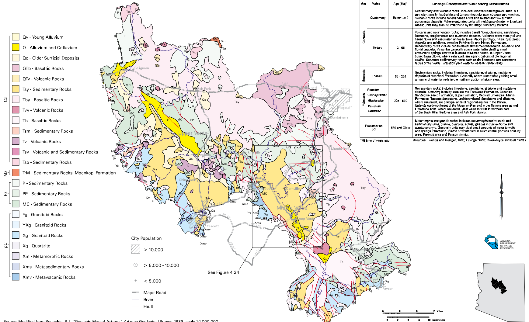
Figure 2.6 - Geology in the Verde River Watershed Study Area
