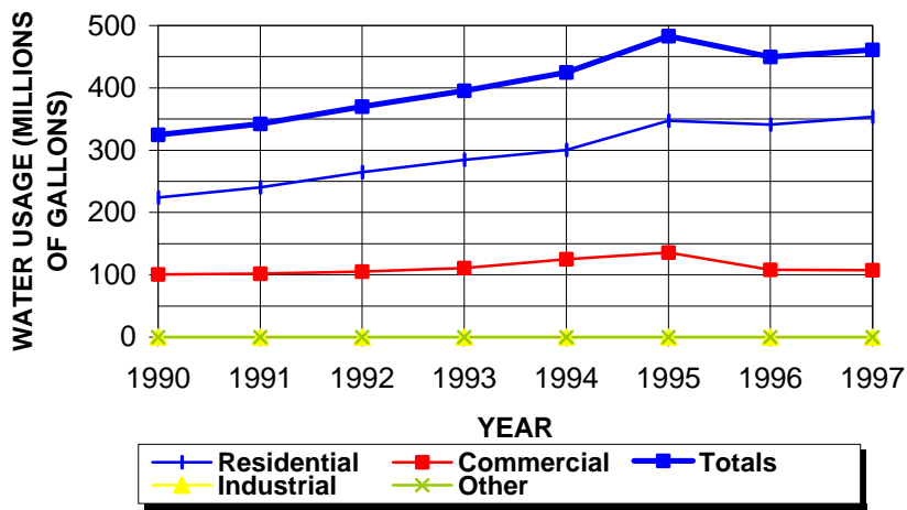
RESIDENTIAL, COMMERCIAL, INDUSTRIAL, OTHER & TOTAL WATER USAGE OVER TIME
