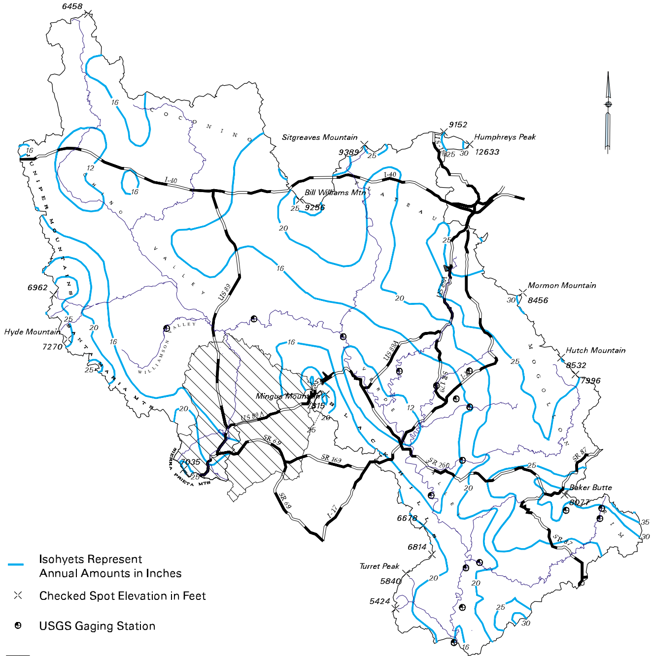
Figure 4.2 - Precipitation in the Verde River Watershed Study Area
