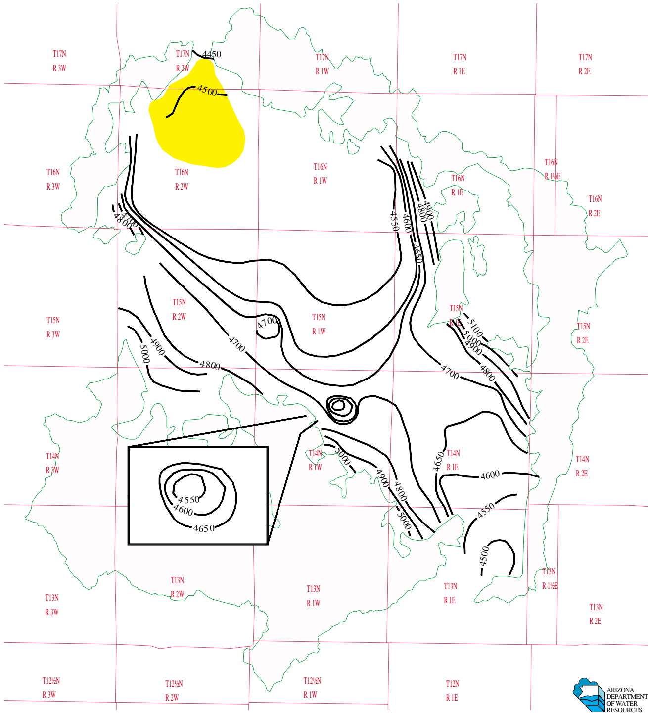
Figure 4.13 –Groundwater Elevations (1994) Prescott Active Management Area
