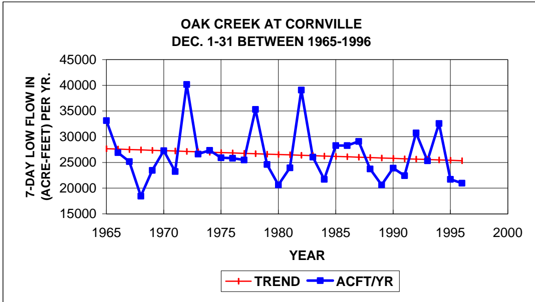
Figure 4.33 Continued Oak Creek At Cornville Gaging Station Dec. & June 1965-1996
