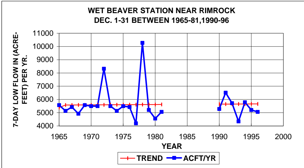
Figure 4.33 Continued Wt. Beaver Station Near Rimrock Dec. & June 1965-1981,1982 & 1990-1996
