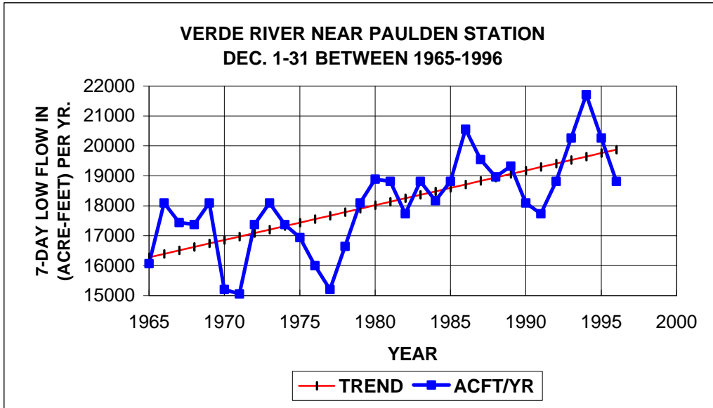
Figure 4.33 Linear Regression Analysis Verde River Near Paulden Gaging Station Dec. & June 1965-1996
